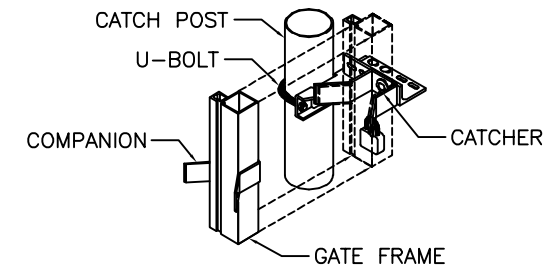
6 CATCH ASSEMBLY SCALE: NTS
