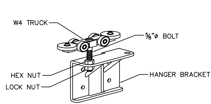
4 GATE HANGER ASSEMBLY SCALE: NTS
