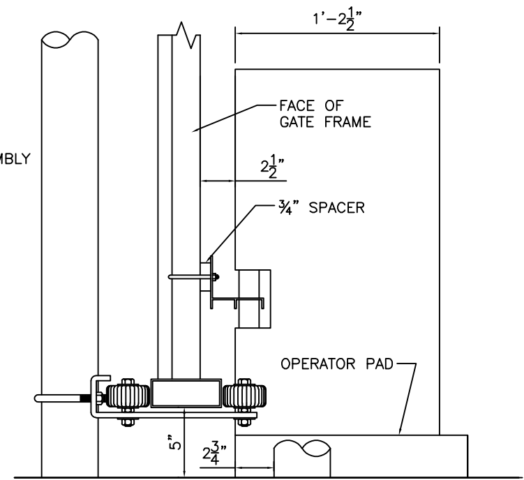
3 OPERATOR SIDE ELEVATION SCALE: NTS
